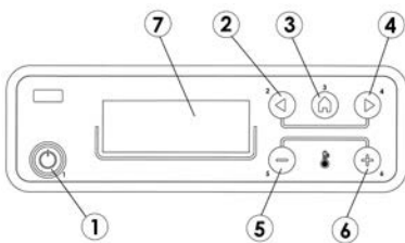
Fig. 7 - Control panel
