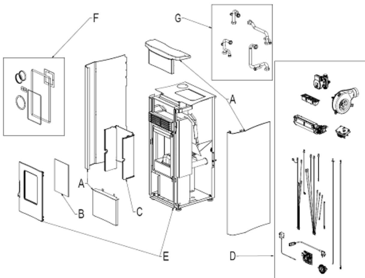
Fig. 1 - Exploded drawing
